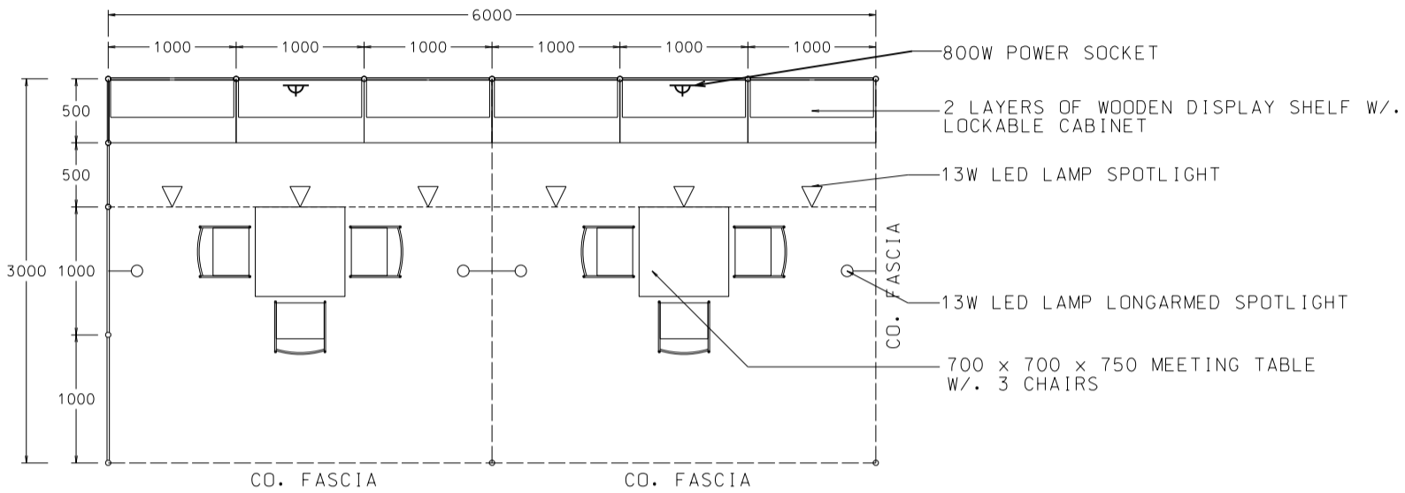
PLAN
