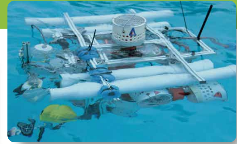
Contact 聯絡: justinah@theiet.org Product 產品: "Alphatar" (The IET / MATE Hong Kong Underwater Robot Challenge 2012 champion by CMA Secondary School)
